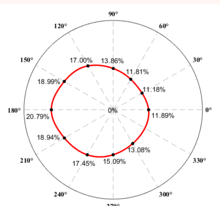
Fig.6: Average Weber fraction
