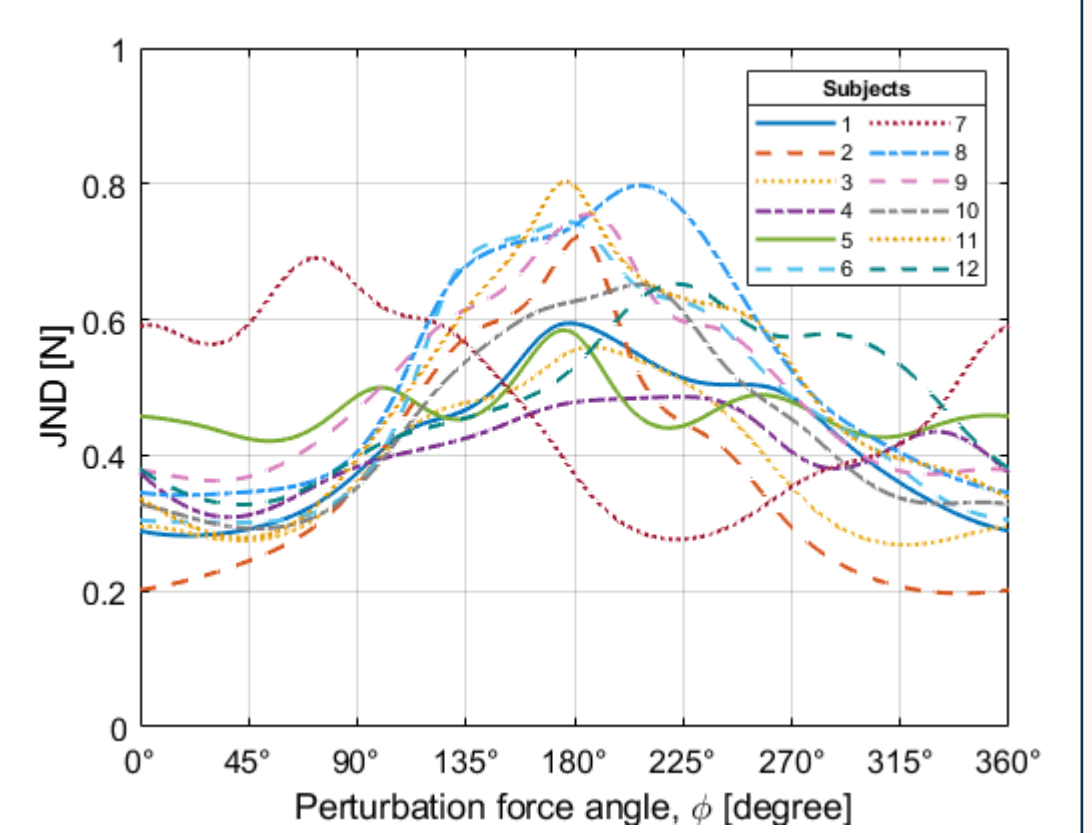
Fig.5: Force JND vs perturbation force angle ( \phi )
